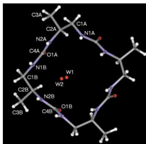
Figure 1. Ball and stick representation of 1 showing the numbering scheme. The torsion angles [ ^\circ ] of the main chain are : N1A-C1A-C2A-N2A 57.9(2), C1A-C2A-N2A-C4A -156.7(2), C2A-N2A-C4A-N1B 177.4(2), N2A-C4A-N1B-C1B 172.6(2), C4A-N1B-C1B-C2B 78.0(3).
